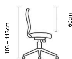
Firefly Task
